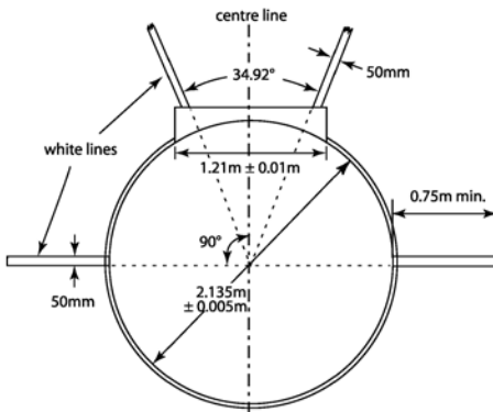
Figure 187A - Layout of Shot Put circle
