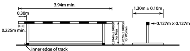
Figure 169a - Example of a steeplechase hurdle
